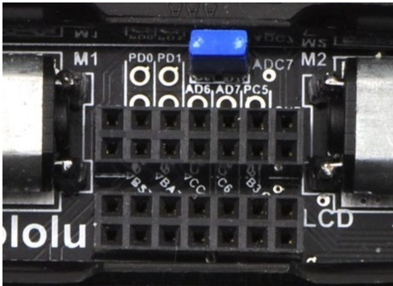
A 2×7 female header soldered into the 3pi expansion pin holes.
