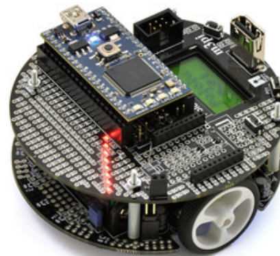
Pololu m3pi robot controlled by an ARM mbed development board.
